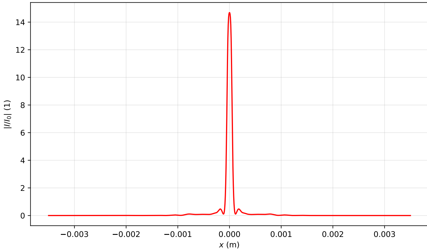
Intensity profile I(x, y = 0, z = 1.194)/I_0 , P_{in}=7.5P_{cr} , artificial time
